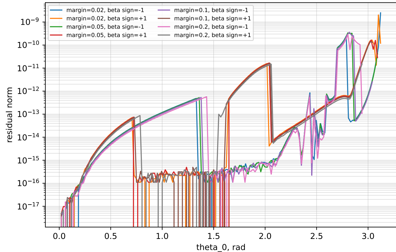
Kappa 1 Residual Norm
